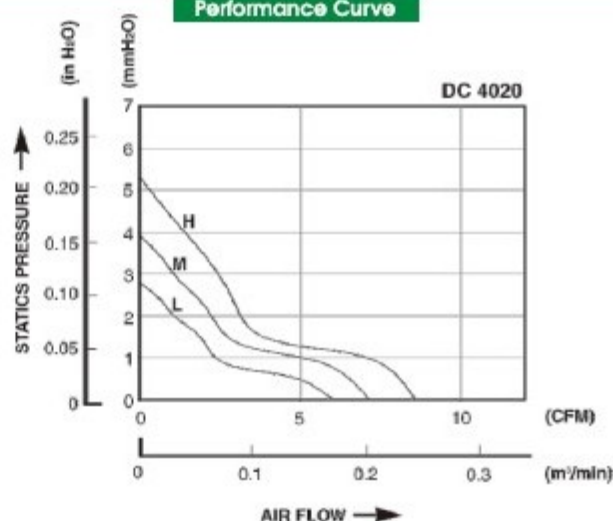
Performance Curve
